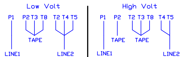
wiring diagram
